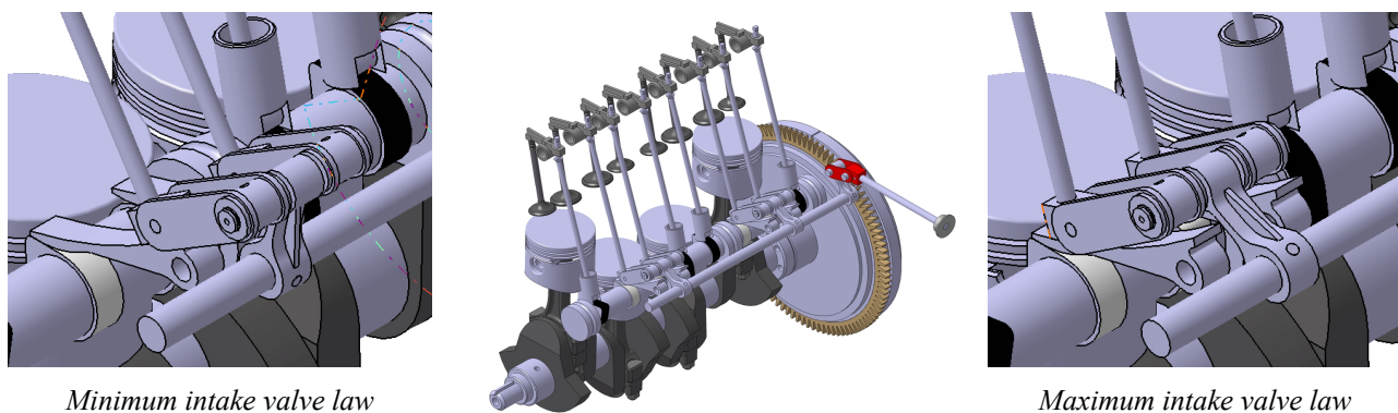
Figure A1. The VVA mechanism featuring side mounting camshaft and overhead valves.
