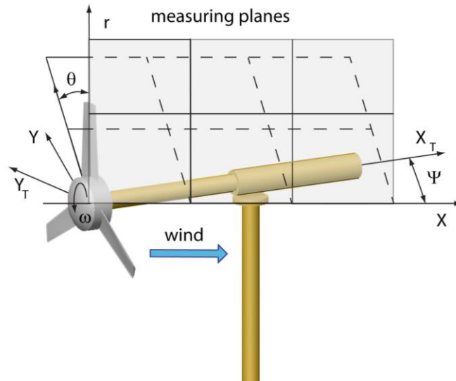
Figure 1 Wind turbine test bench
