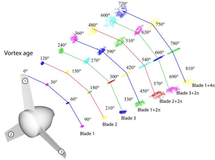
Fig. 5 Vortex center positions.
