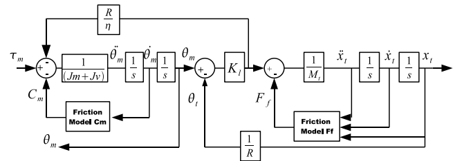
Fig. 2. Mechanical subsystem
