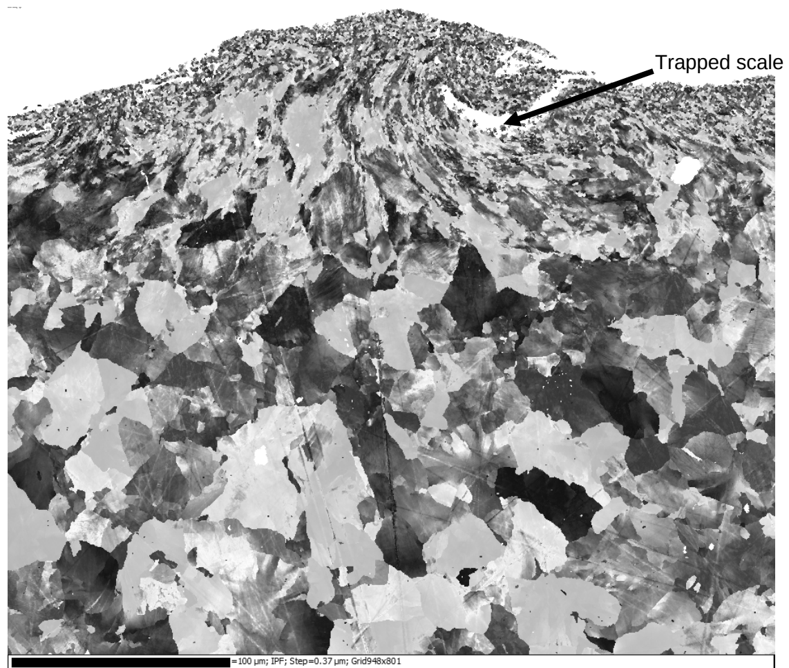
Fig 4 EBSD image of the first 300 \mu m in a shot-blasted connecting rod. Scale has been trapped in a 50 \mu m fold during the shot-blasting.
