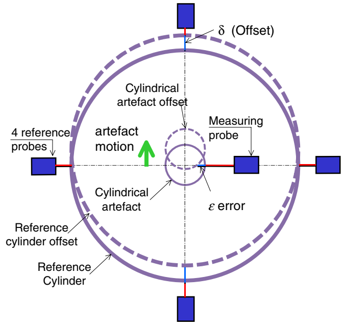
Figure 9. Description of the compensation of the probe offset error.
