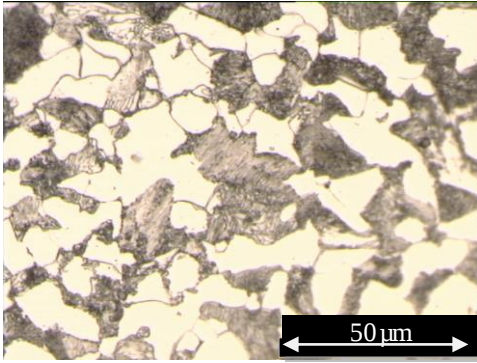
Figure 3. Microstructure of as-received C38 (Becker, Arts et M é tiers ParisTech).
