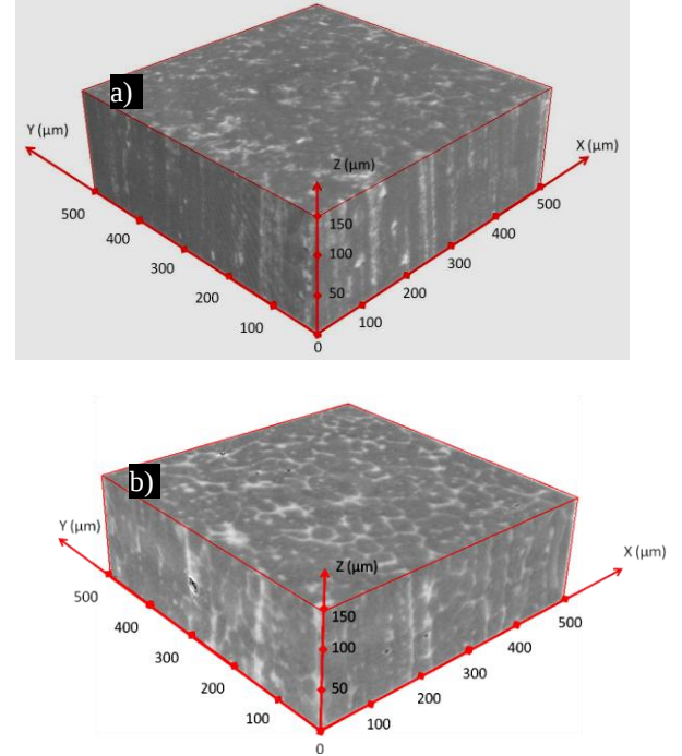
Figure 8. 3D representation of M2 steel in (a) as-received state, and in (b) partial remelted state. Volume = 0.5\text{mm} \times 0.5\text{mm} \times 0.15\text{mm}
