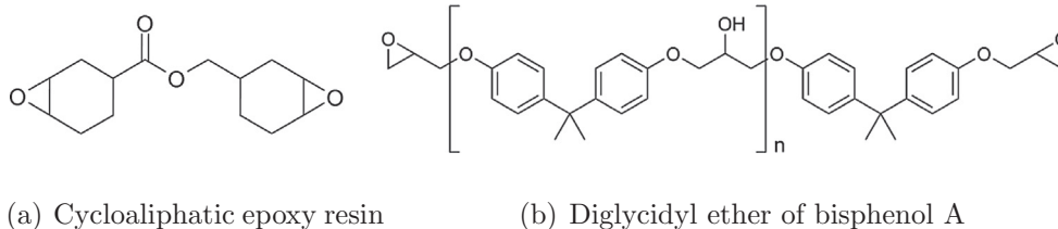
Fig. 1. Main epoxy monomers in the resin part of EPOLAM 2063.
