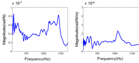
Fig. 7: The calculated h_{BB,uu}^2 and h_{BB,\theta\theta}^2 of the System 2
