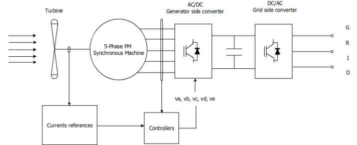
Fig. 1. General scheme of the tidal system.
