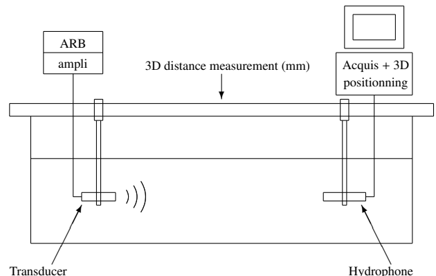
Figure 1: Experimental configuration
