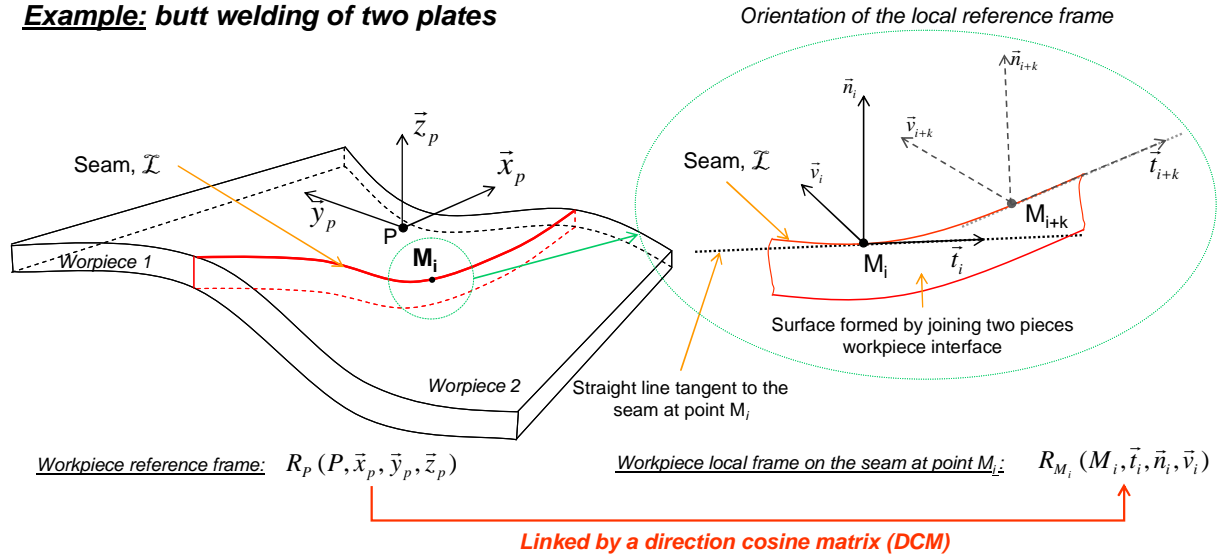
Figure 3: Definition of the seam local frame orientation
