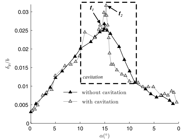
Fig. 20. Effect of cavitation on maximum displacement, \dot{\alpha}^* = 1.89 , Re = 750\,000 , V_\infty = 5\text{ m/s} , \sigma = 3 : cavitation; \sigma = 7 : without cavitation.
