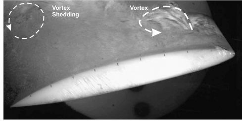
(g) \alpha^- = 14^\circ .
