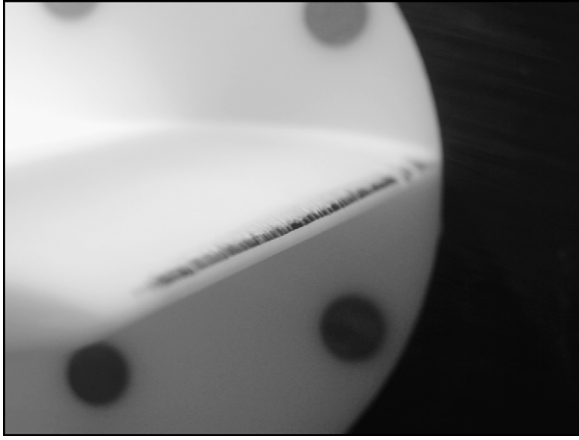
Fig. 11. Cavitation at inception at the leading edge for a fixed angle of incidence, \alpha = 8^\circ , \sigma = 3 , Re = 750\,000 , V_\infty = 5\text{ m/s} .
