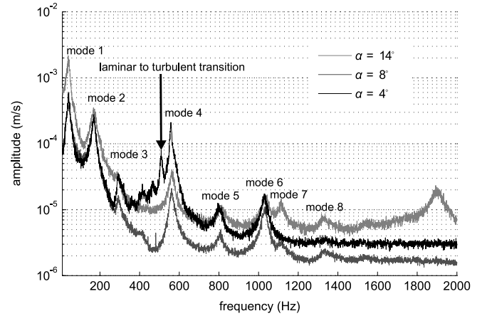
Fig. 7. Velocity spectrum for various angles of incidence, static case, Re = 750\,000 , V_\infty = 5 m/s.
