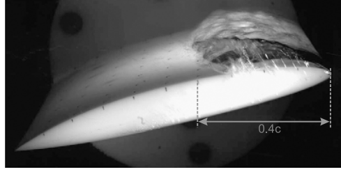
(c) \alpha^+ = 14^\circ .
