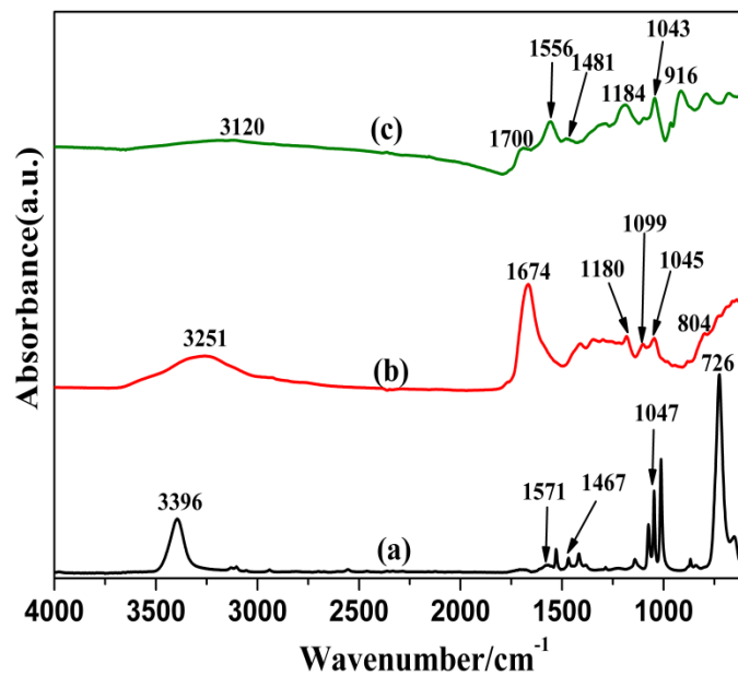
Figure 4. ATR-FTIR spectra of pure pyrrole before polymerization (a), radiolytically synthesized PPy after lyophilization (b), and chemically synthesized PPy after lyophilization (c).
