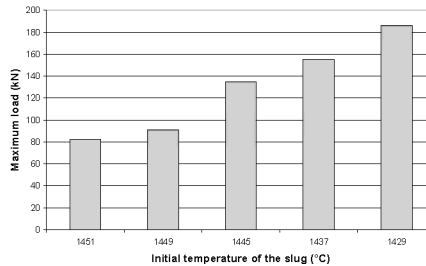
Figure 5. Maximum load to obtained part by changing initial temperature of the slug
