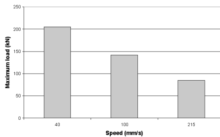
Figure 4. Maximum load to obtain the part for each speed.
