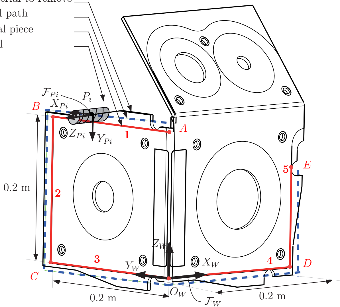
Figure 3.1 – Workpiece
