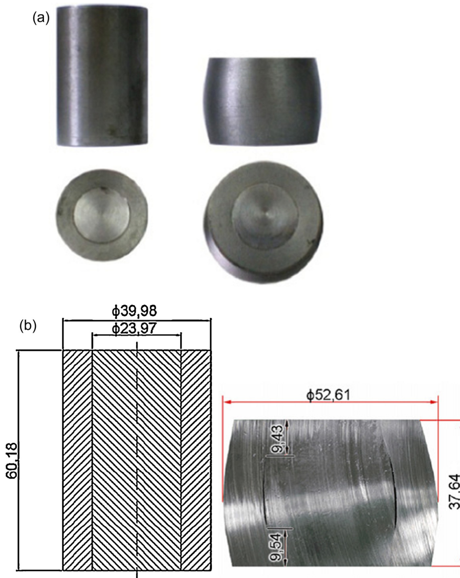
Fig. 4. Initial and compressed billet (a) initial and compressed bi-metal ring and (b) meridian cross section of bi-metal ring after compressed ( Essa et al., 2012 ).
