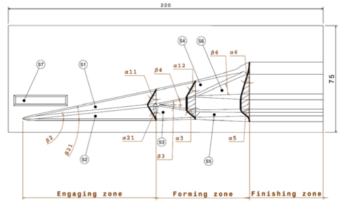
Figure 4. Geometry of one half of the experimental flat dies (symmetry)
