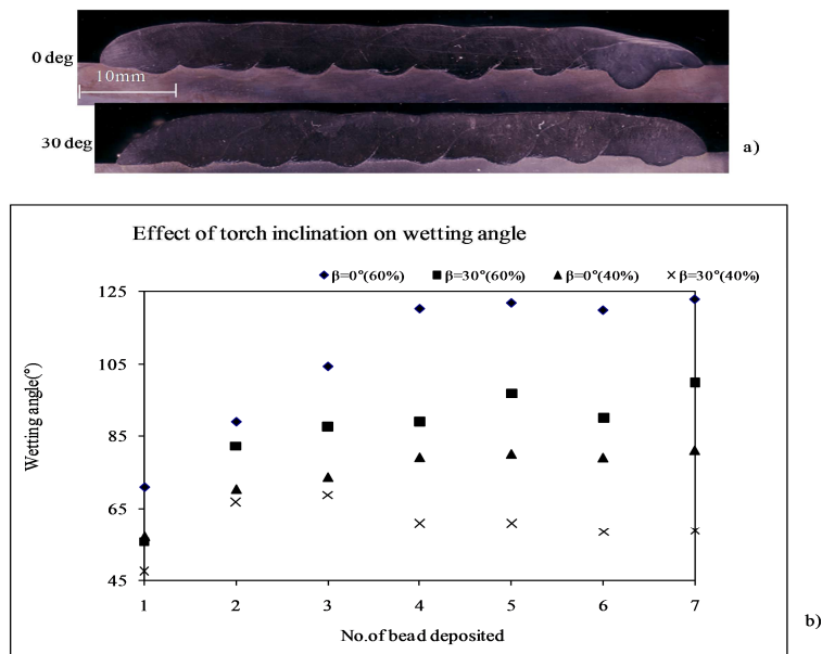
FIGURE 6 Macrographs of cladbed beads at different torch angles (a) and its effect on wetting angle (b)
