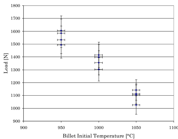
FIGURE 5. Loads measured at stroke x = 56mm for various initial billet temperatures
