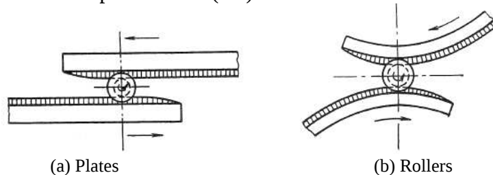
FIGURE 1. from HOLUB 1972 [1]: Most common configurations used in cross wedge rolling Industrial applications for steel parts are achieved at hot temperatures either for preforming operations or for semi-finished parts. Among different condition, a
