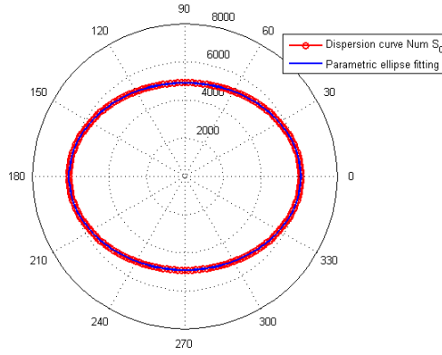
Figure 11: Dispersion curve for the new material and its corresponding parametric fit
