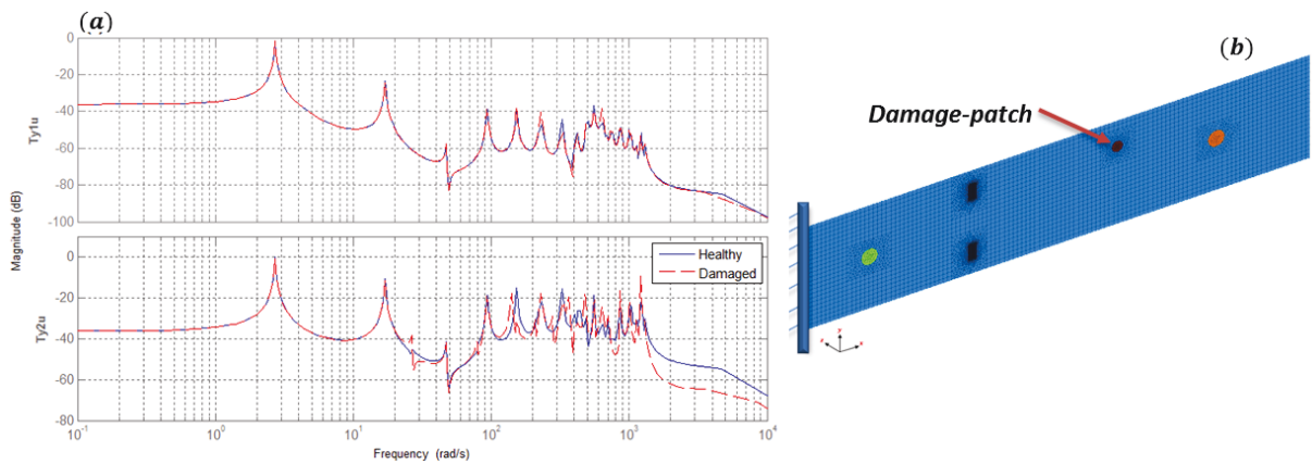
Fig. 13: (a) Comparing the effect on the complete model including a small damage. (b) BVID Damage centered at position (x = 570, y = 140) mm
