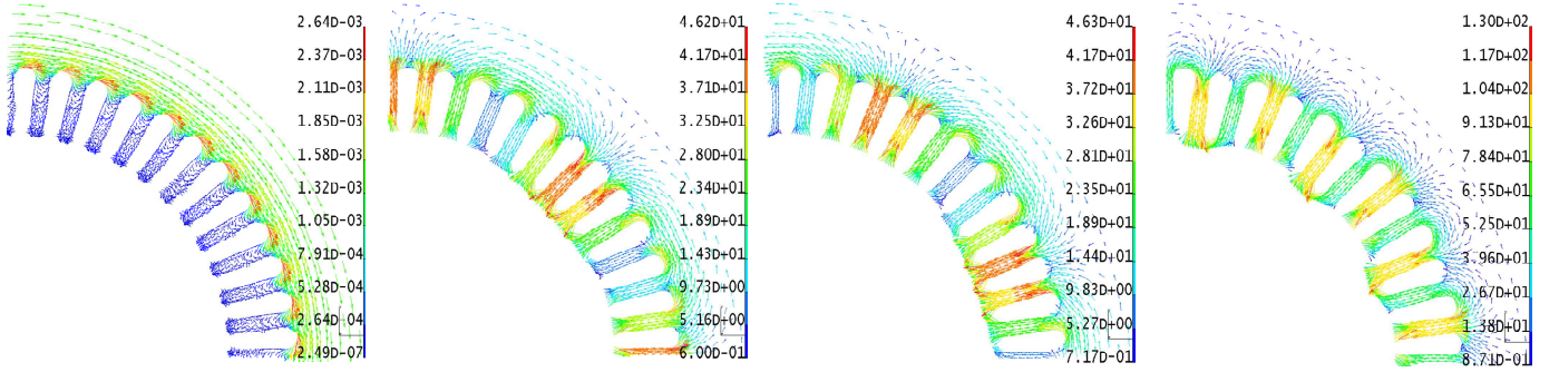
Figure 8: Distributions of \text{curl } \Psi_i for i=\{1,4\} obtained from the second configuration
