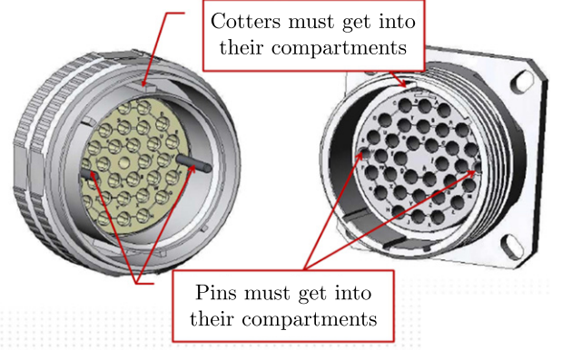
Fig. 3. Electrical connector.
