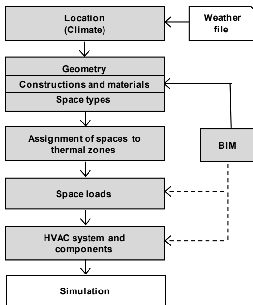
Figure 4. An ideal workflow for energy performance in thermal simulation tools [5].
