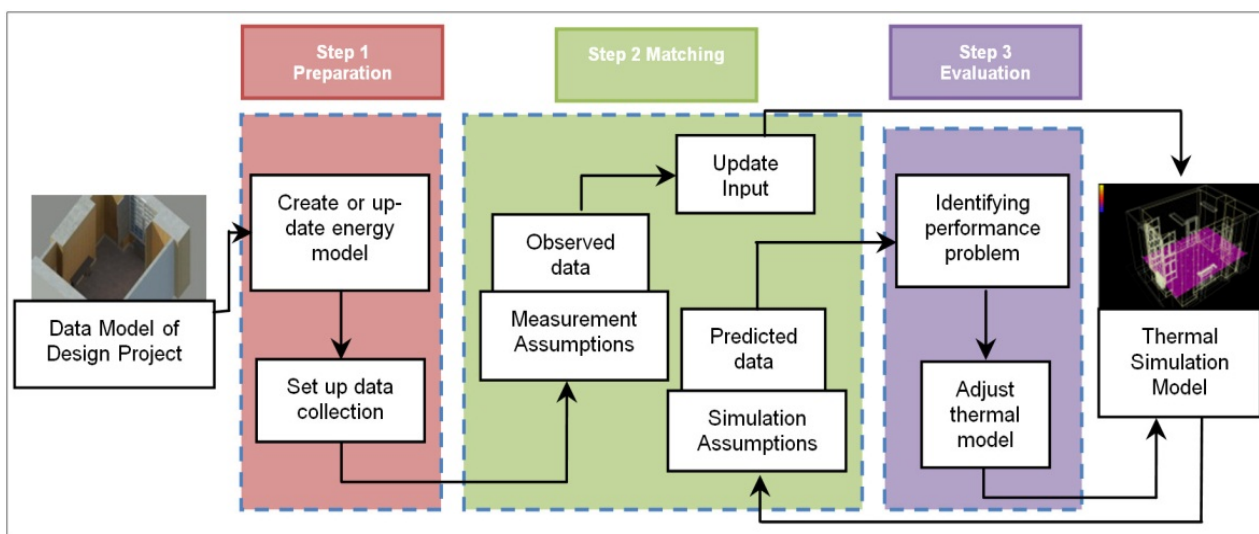
Figure 2. Workflow to produce a thermal simulation model.
