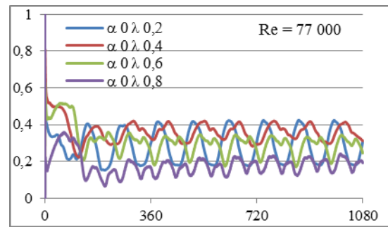
Fig. 20 Re=77\,000 , \alpha=0 degree
