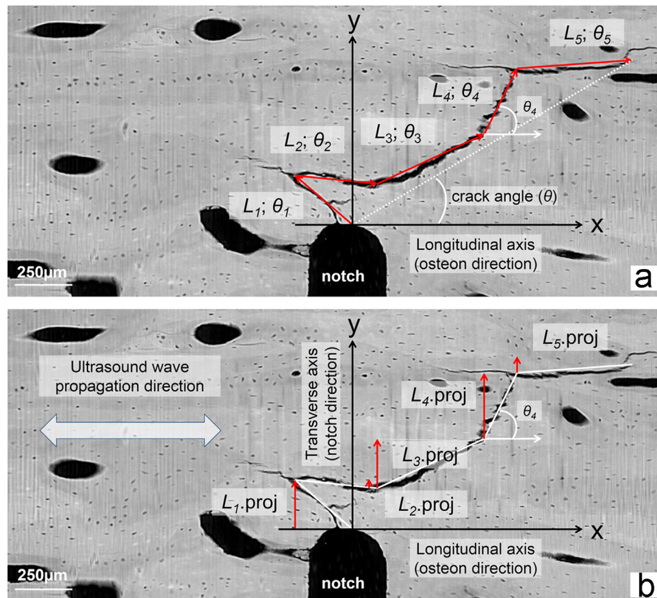
Fig. 3 – (a) Decomposition of the main crack into 5 vectors with lengths L_n and angles \theta_n . The crack length Cr.Le = L_1 + L_2 + L_3 + L_4 + L_5 . The mean crack angle is estimated in a coordinate system composed by the osteon direction (x axis) and the notch direction (y axis). It corresponds to the vector orientation between both extremities of the main crack. (b) The orthogonal projection of the main crack on the transverse axis corresponds to the sum of the 5 vectors projected on the same axis. Cr.Le.Proj = L_1.Proj + L_2.Proj + L_3.Proj + L_4.Proj + L_5.Proj (with L_n.Proj = L_n \cdot \sin(\theta_n) ).
