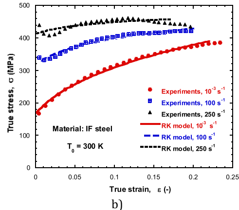
Fig. 5. a) RK model for different strain rates; b) Comparison between RK modeling and experimental data.
