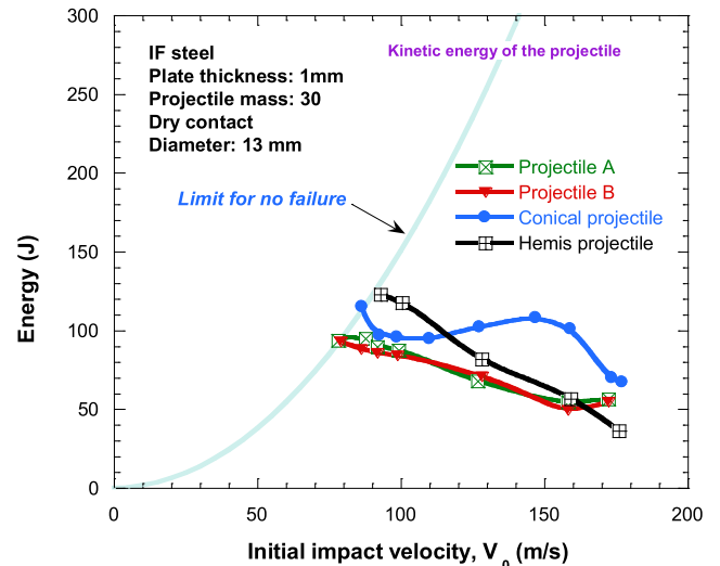
Fig. 10. Experimental results in term of absorbed energy for different projectile shapes.
