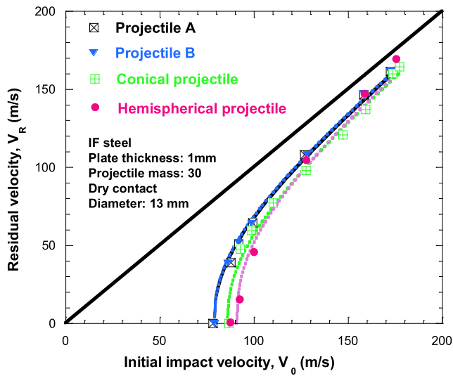
Fig. 9. Experimental results in terms of residual velocities for different projectile shapes.
