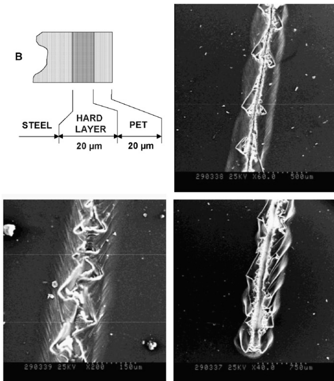
Fig. 5. Constitution and morphologies of scratch on product B; every photo illustrates a different deformation mode—mode I (on top and right: low amplitude ruptures), mode II (on bottom and left: shortcoming increase to critical size) and mode III (on bottom and right: delaminating and remnants).
