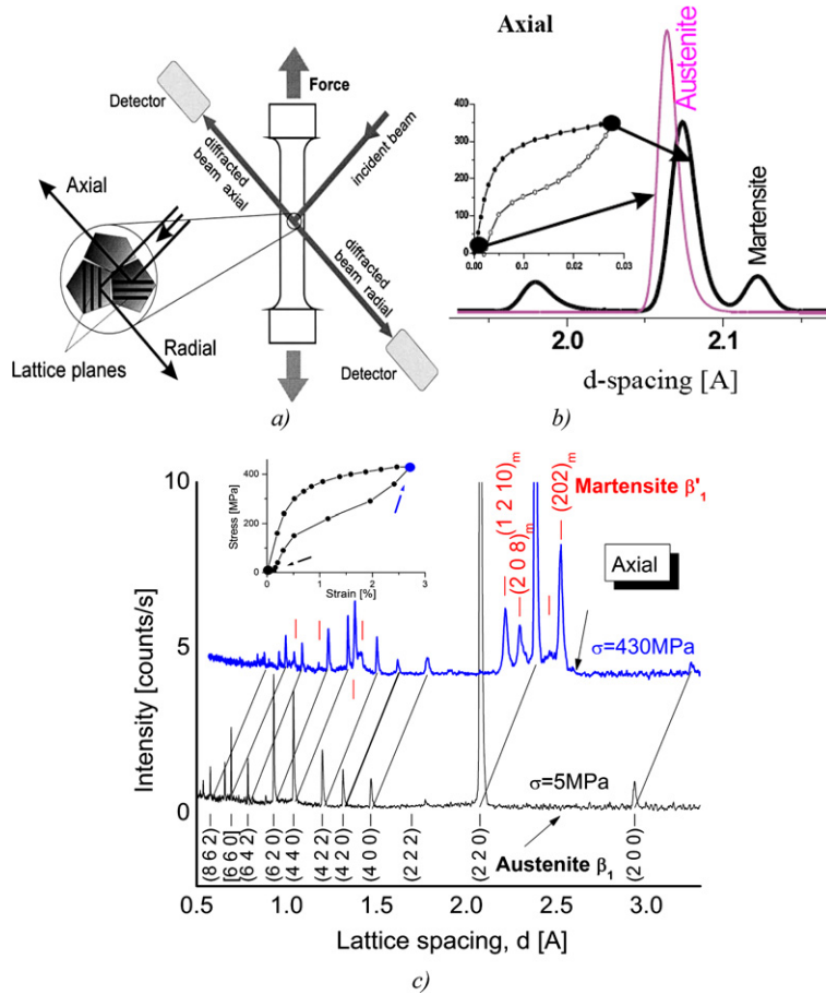
Fig. 2. Principe of in situ neutron diffraction measurements on polycrystalline SMAs: a) the specimen (gauge volume \sim \text{cm}^3 ) is loaded mechanically inside the neutron diffractometer. The neutron spectra at fixed angular position are recorded by two detectors in two geometric configurations denoted as 'axial' and 'radial', in which the diffracting lattice planes are oriented either perpendicular or parallel to the tensile load axis, respectively; b) integral intensities and positions of reflections of the austenite and martensite phases are measured at selected [\sigma, \epsilon, T] states; c) TOF neutron diffraction spectra of the CuAlZnMn polycrystal in the axial configuration recorded in the first cycle under tensile stresses of 5 MPa and 430 MPa at room temperature [7].
