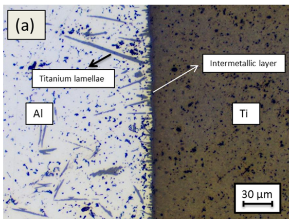
Fig. 10. Close-up of the intermetallic layer: (a) sample 1 (56.24J/mm, 0.75 mm) with straight intermetallic interface, (b) sample 9 (65.62J/mm, 0.75 mm) with irregular growth of the intermetallic layer.
