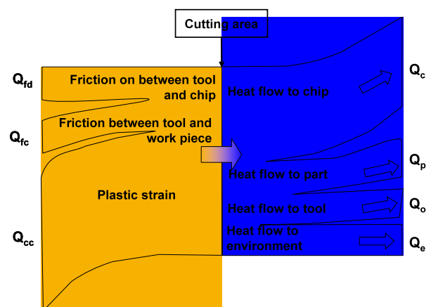
Figure 2: Heat sources and distribution during machining
