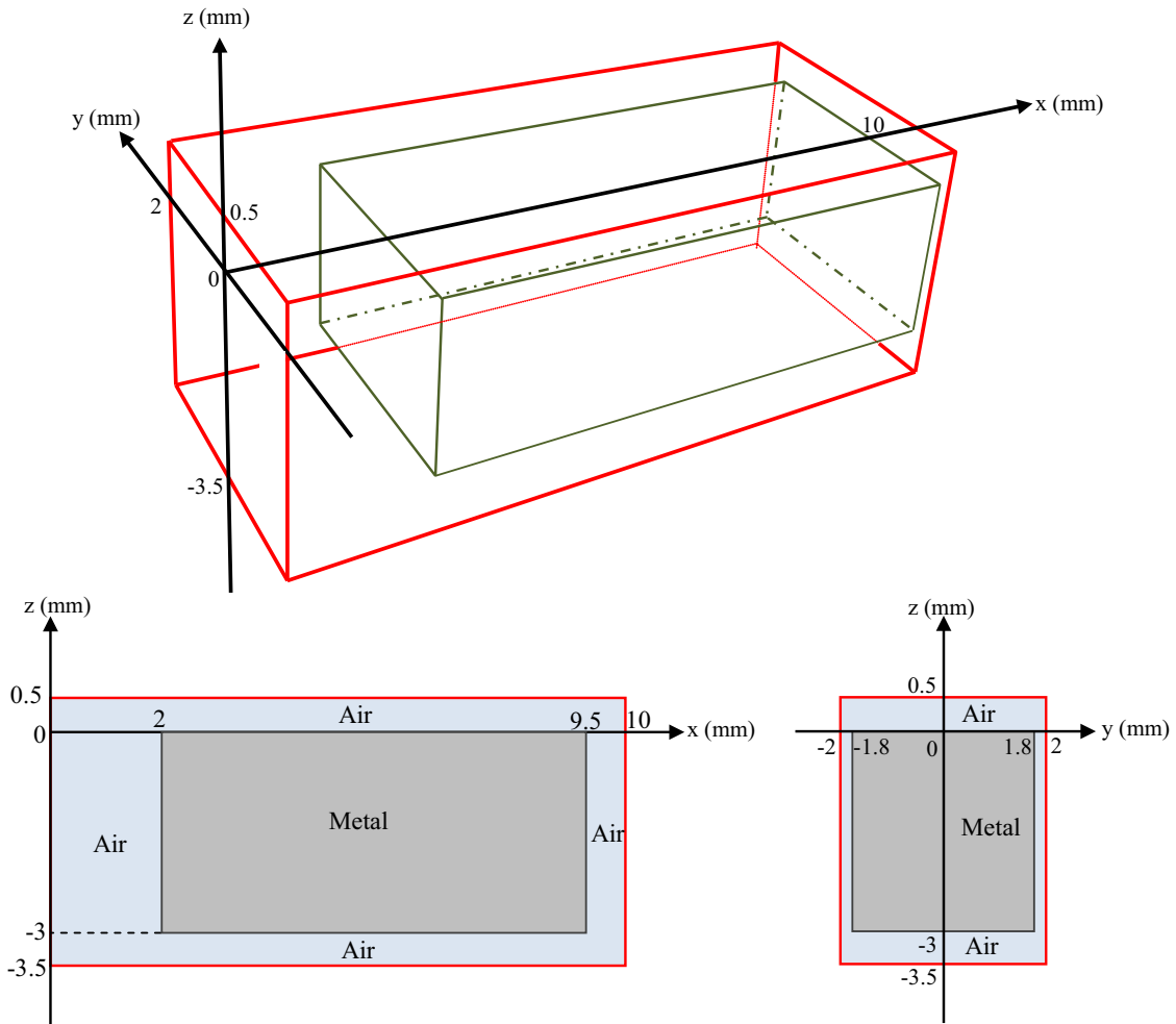
Fig. 5 Calculation field dimensions
