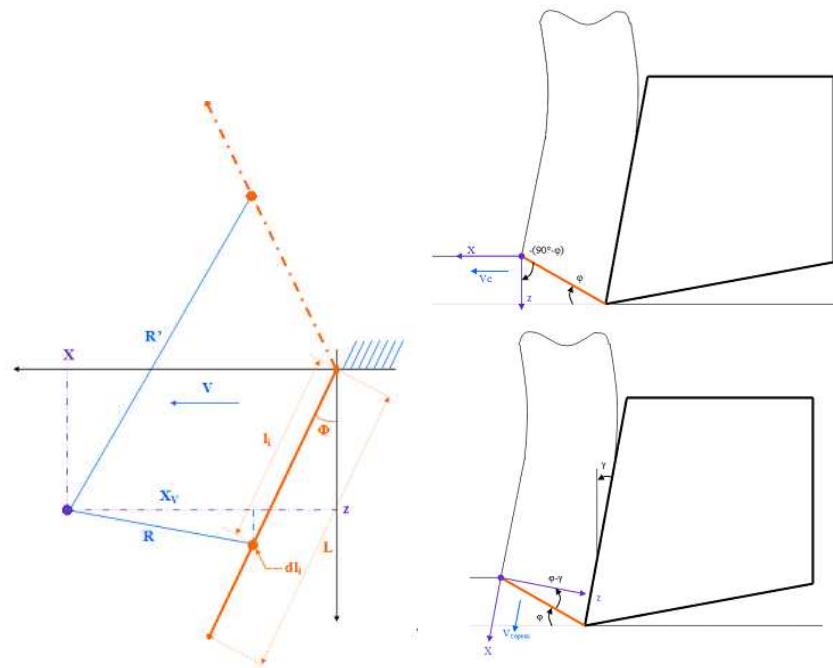
Figure 1 - Simplified analytical modelling of the primary shear zone
