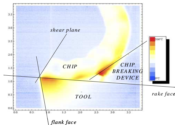
Figure 4 – Thermal image recorded free cutting steel – V_c = 110 \text{ m/min} – f = 0,4 \text{ mm/rev} – a_p = 1,5 \text{ mm}
