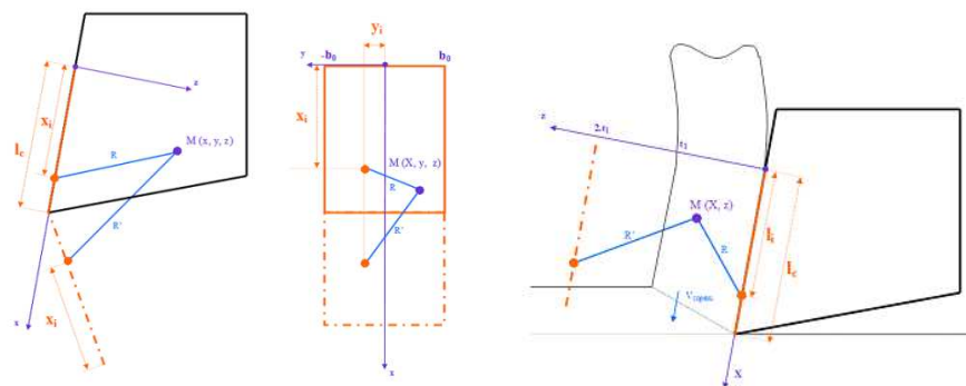
Figure 2 - Simplified analytical modelling of the secondary shear zone
