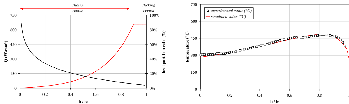
Figure 5 – Temperature distribution and heat flux free cutting steel – V_c = 110 m/min – f = 0,4 mm /rev – a_p = 1,5 mm
