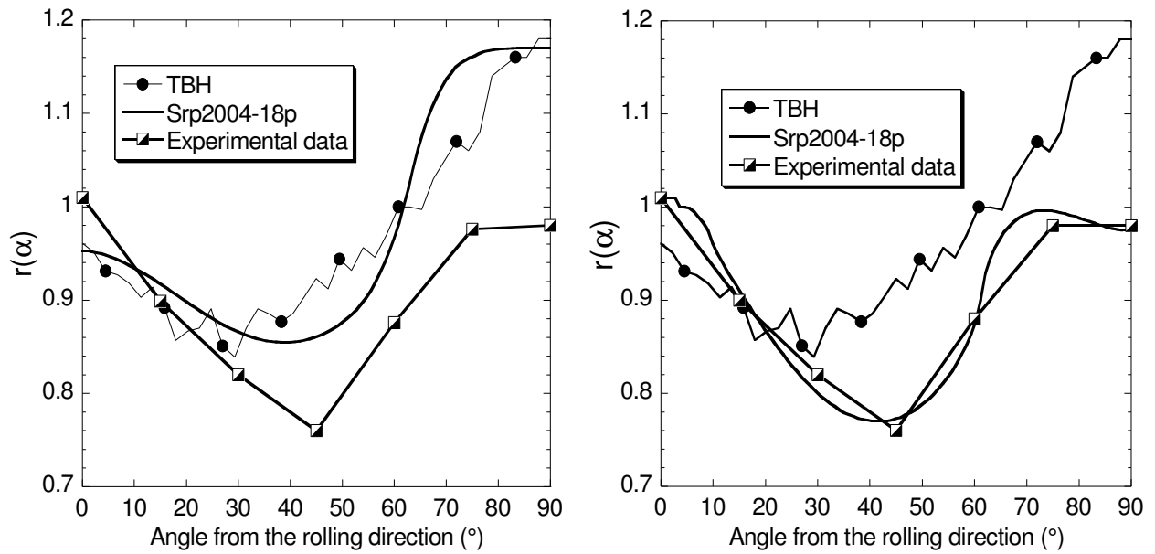
Figure 12. Impact of the identification technique on the predicted r -values for the Srp2004-18p potential and comparison to experimental and micromechanical results; a) identification using texture data, and b) identification using experimental data from mechanical tests.
