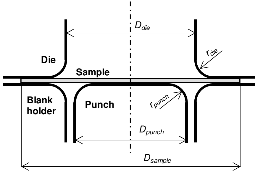
Figure 1. Cup drawing test geometry.
