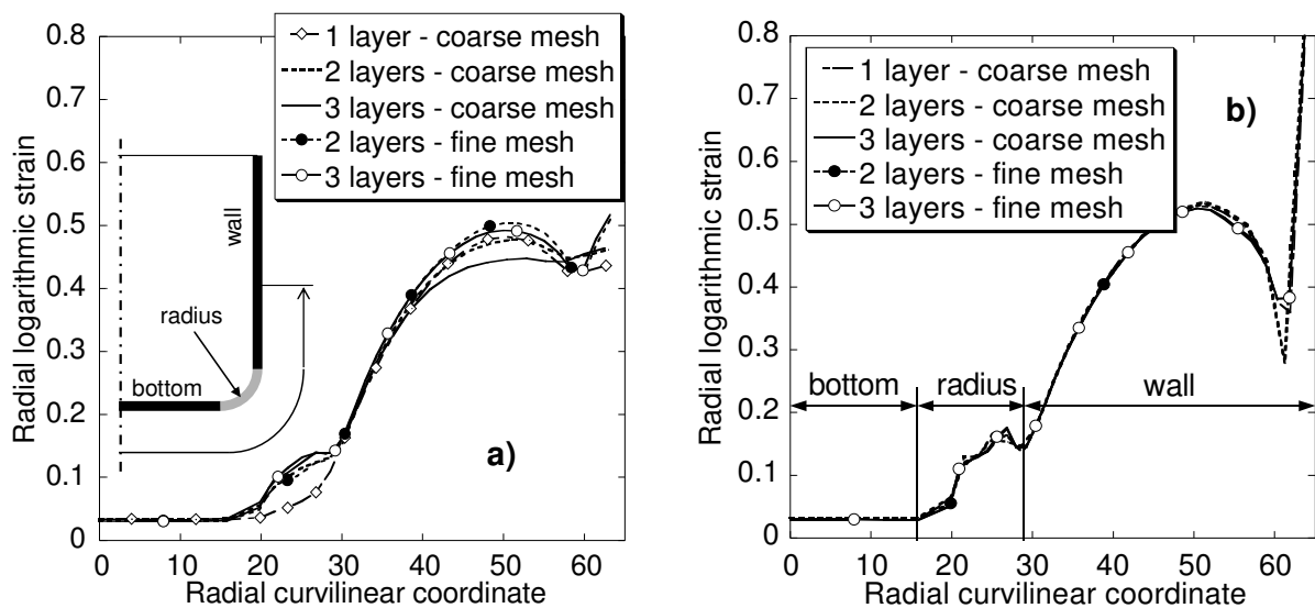
Figure 4. Radial strain distribution along the rolling direction predicted with the different meshes using: a) the reduced integration element C3D8R, and b) the hybrid element with incompatible modes C3D8IH.
