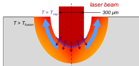
Figure 1: Schematic view of the drilling process
