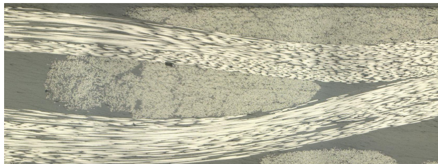
Figure 4 Details of the interlock 3X 55% woven composite microstructure
