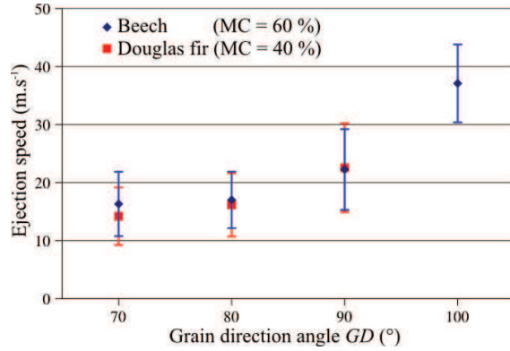
Figure 9: Chip ejection speed function of grain direction angle. Mean and standard deviation of 100 values. ( b = 10 mm, h = 10 mm)
