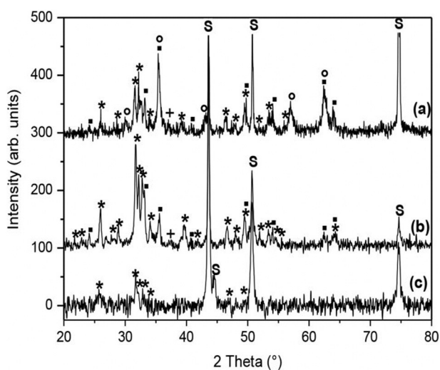
Fig. 2. XRD patterns of the different HAP coatings formed on the 316 L SS: (a) 50 mm/min, 700 °C – 60 min, (b) 50 mm/min, 600 °C – 60 min, (c) 80 mm/min, 500 °C – 60 min. (■) \text{Fe}_2\text{O}_3 , (+) \text{Fe}_3\text{O}_4 , (*) \text{FeCr}_2\text{O}_4 , (S) Substrate.
