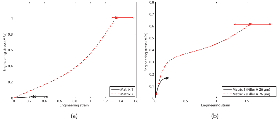
Figure 4: Uniaxial tension behaviors of two propellant matrices (a) and of the two corresponding propellants filled with filler A (b).
