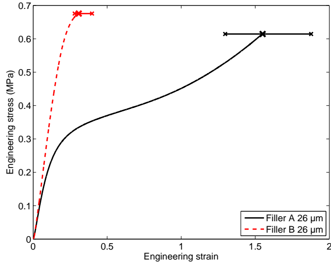
Figure 3: Uniaxial tension stress-strain behavior of filler A or B filled propellants illustrating the impact of the nature of the adhesion at the filler/matrix interface.
