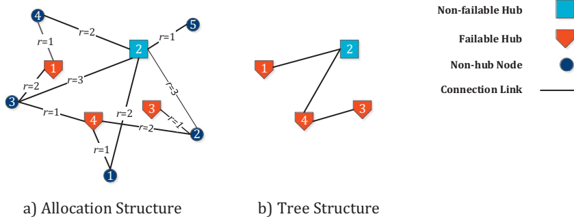
Fig. 1. Logistics of the proposed RHLP.
