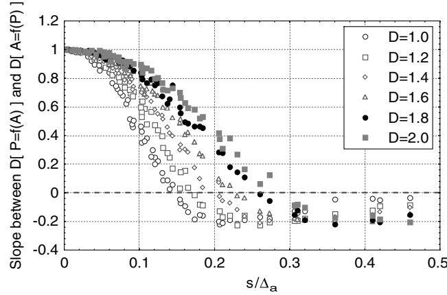
Fig. 4. Master curve of the slope between \Delta_{P=f(A)} and \Delta_{A=f(P)} versus the ratio s'_e/\Delta_a for fractal dimension varying between 1 and 2. All Monte-Carlo configurations are considered.
