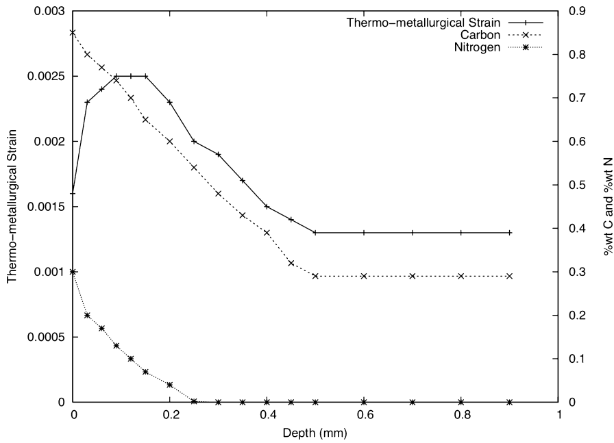
Fig. 13. Carbonitrided specimen: in-depth thermo-metallurgical strain profile (component xx ) depending on the percentage of carbon and nitrogen at 25^\circ\text{C} (results obtained using JMatPro).
