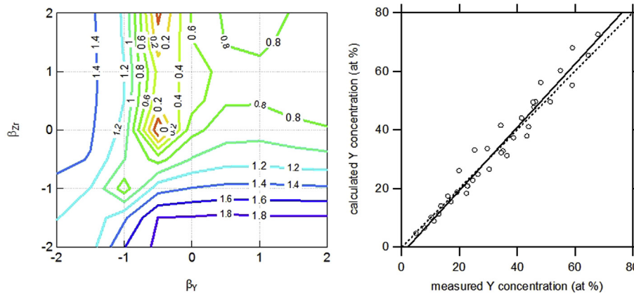
Fig. 3. Left. Optimization of the angular distributions for Zr and Y. The figure shows the relative error between the measured and simulated composition as a function of \beta for Zr and Y. \beta defines the angular distribution of the sputtered atoms as defined by Eq. (1). Right. Correlation between the measured and simulated composition for the optimized condition, i.e. \beta_Y = -0.5 and \beta_{\text{Zr}} = 0 . The striped line corresponds to the 1:1 correlation, while the full line is a linear fit through the data points.
