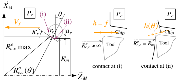
Fig. 1. Representation of the R_{c,c}^o radius in cylindrical turning [13].
