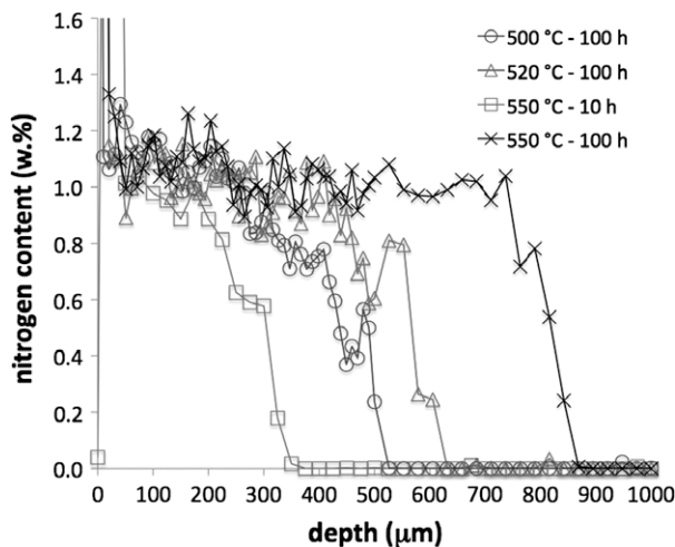
Fig. 1. Influence of process temperatures and times on nitrogen diffusion of nitrided Fe-3%Cr-0.35%C (EPMA analyses).
