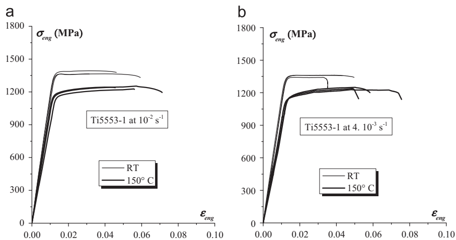
Fig. 8. Effect of the temperature on the engineering stress–strain curve: (a) Ti5553-1 at 10^{-2} \text{ s}^{-1} ; (b) Ti5553-1 at 4 \cdot 10^{-3} \text{ s}^{-1} .
