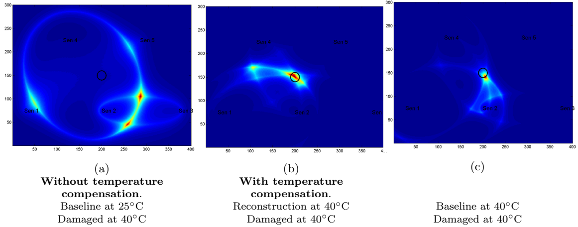
Figure 17: Damage imaging of the composite laminate at 40°C, black circle represents true damage location. Numerical study
