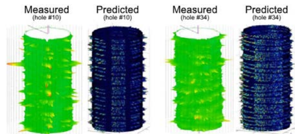
Fig. 10. Measured and predicted distribution of the uncut fibers around the holes for MD CFRP (20  m/div), after hole number #10 and #34.
