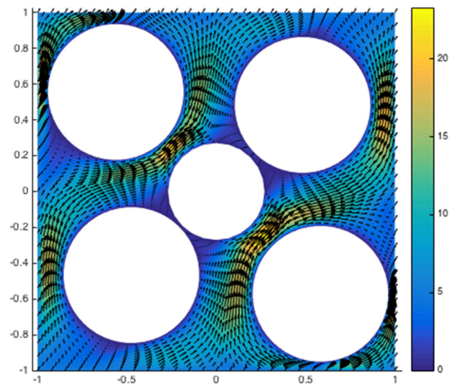
Fig. 3 Microscopic velocity field \mathbf{v}(\mathbf{x}) associated with the macroscopic velocity field \mathbf{V}^T = (V \cos \theta, V \sin \theta) , V = 5 \text{ mm} \cdot \text{s}^{-1} and \theta = \pi/3
