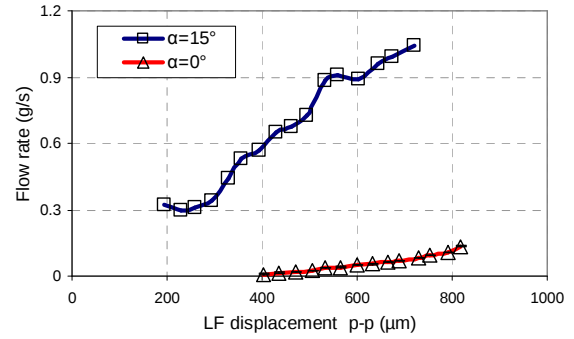
Fig. 5. Flow rate in function of LF displacement for different inclination of the system using a corundum powder. Stainless steel quality of the beam surface.
